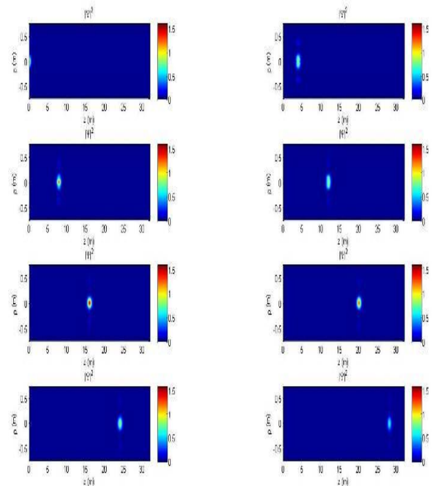
Figure 6: (Color online) As a second application of our method to ultrasonic (acoustic) pulses, let us consider now a truncated Bessel pulse with an initial spot-radius of 23 cm, generated by a finite antenna still with radius R = 0.5 m. Attenuation (actually strong for a 40 kHz frequency) is neglected again. We wanted our realistic pulse to keep its spot size unvaried for the larger distance of about 30 m. The present set of figures, representing by colors the actual pulse evolution, does indeed show such a behavior.
