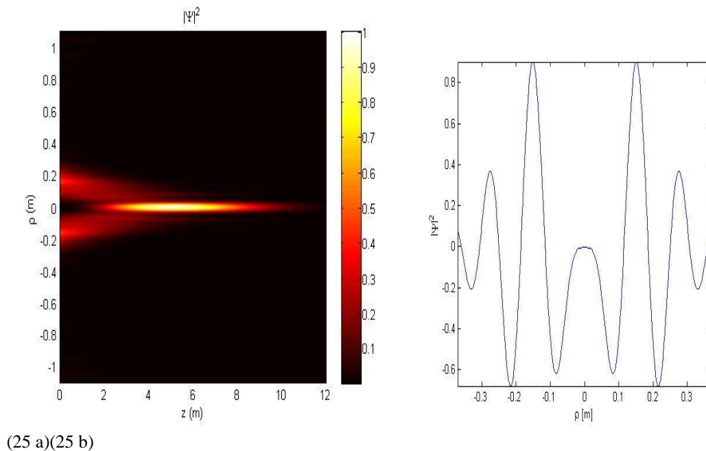
Fig. 25 – Our theoretical method[20,4,2] allows constructing an acoustic Frozen Waves with the characteristics specified in the Example above. This is shown in the present Figure.
