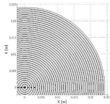
Fig. 19 – Example of an acoustic annular aperture having a radius of 24.5 mm and 41 rings (with width \Delta d = 0.1 mm, and inter-ring distance d = 0.5 mm). The figure shows the section of the annular transducer array chosen for producing FWs of 1.5 MHz.
