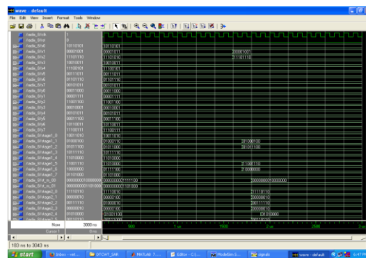
Fig 4.simulation waveform of 8-pt FFT
