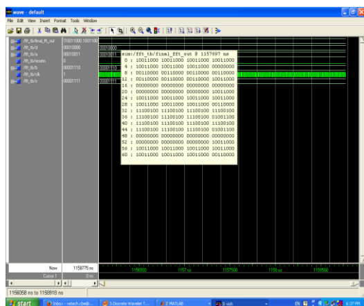
Fig 4.simulation waveform of 8-pt FFT
