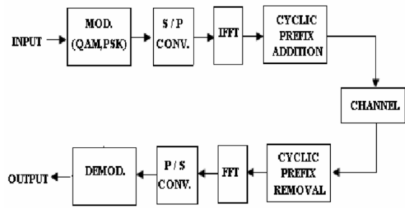
Fig. 3. Block diagram of OFDM transceiver
