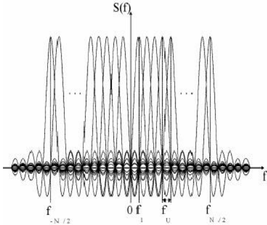
Fig.2.OFDM Subcarrier in Frequency Domain
