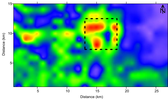
Figure 5. Analytic signal map of the study area.
