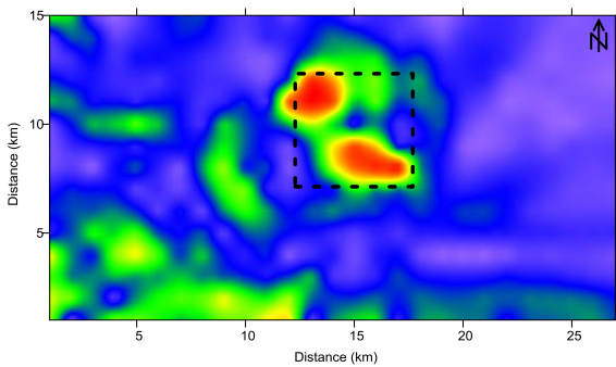
Figure 6. Maximum horizontal gradient map of the study area.
