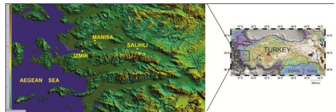
Figure 1. Location of Salihli geothermal area.
