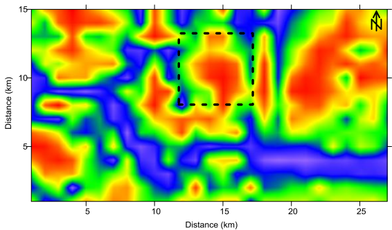
Figure 7. Tilt angle map of the study area.
