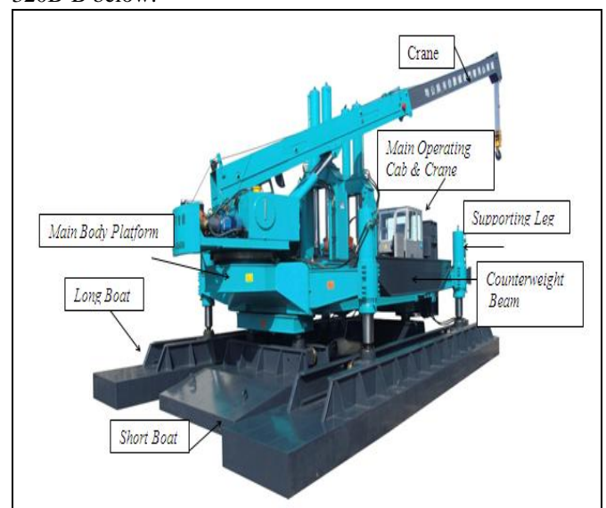
Figure 1. Hydraulic Static Pile Driver Type ZYC 320B-B
