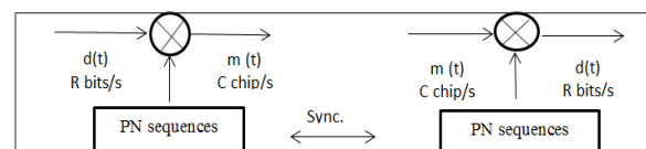
Figure 2. The DSSS technique [10]
