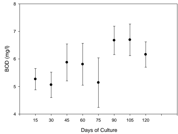
Fig.2.Biochemical oxygen demand
