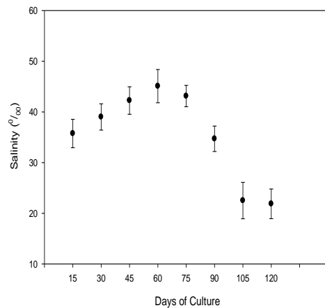
Fig.4.Range of salinity
