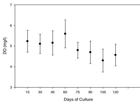
Fig.1.Dissolved oxygen concentration
