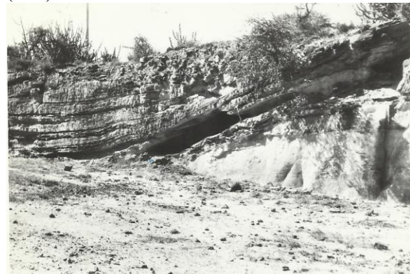
Fig. 2: hummocky cross-stratified bed.
