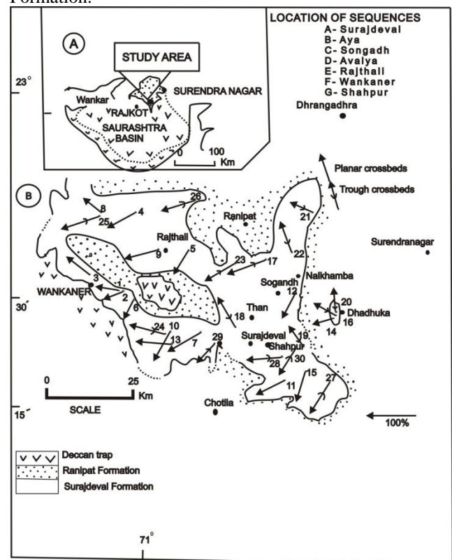
Fig.1A: Geological map of Saurashtra basin.
