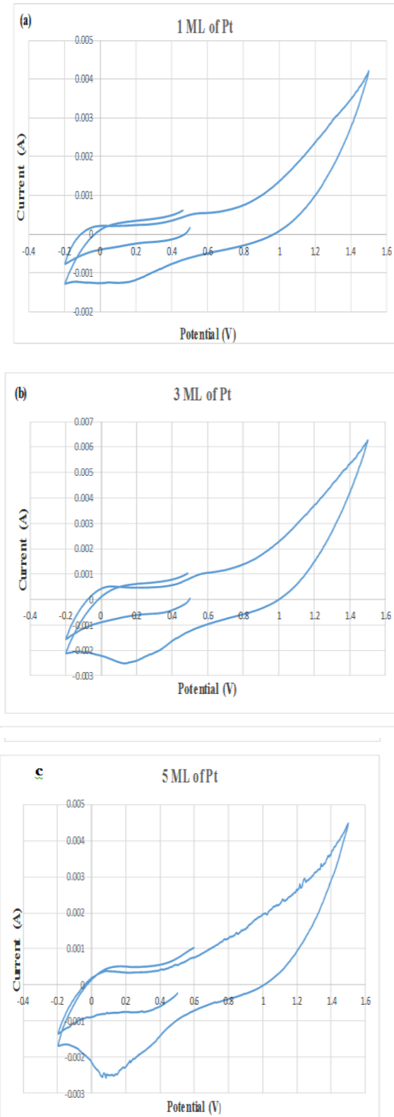
Figure (1.5): CV spectrum for 1,3 and 5 ML samples of Pt deposited on Bucky paper (BP);(a) 1 ML of Pt-BP. (b) 3 ML of Pt-BP. (c) 5 ML of Pt-BP.
