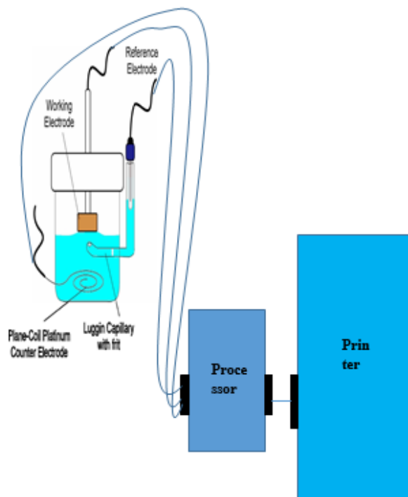
Figure (1.3): Illustration of electrochemical cell geometry employed to Cu UPD step and Pt deposition.
