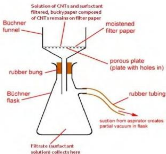
Figure (1.1): A set up of Buchner filtration to filter suspended solution of dispersed CNTs in surfactant solution [12].
