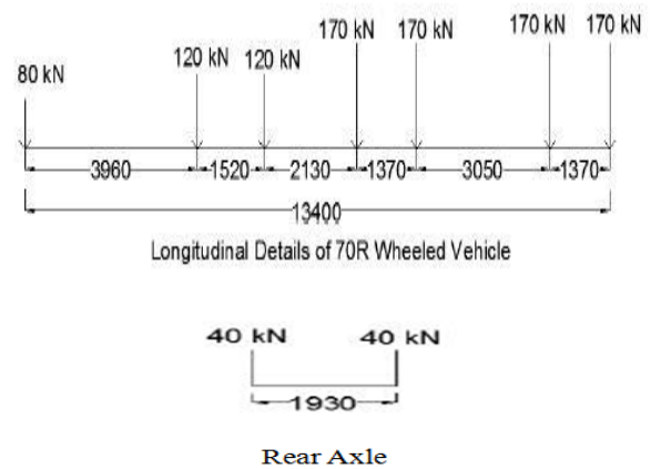
Fig 3: Class 70R Wheeled Vehicle Rear Axle
