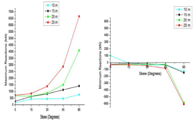
Fig 8: Maximum Positive Reaction Class70RW+A and Maximum Negative Reaction Class70RW+A
