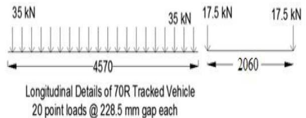
Fig 4: Class 70R Tracked Vehicle
