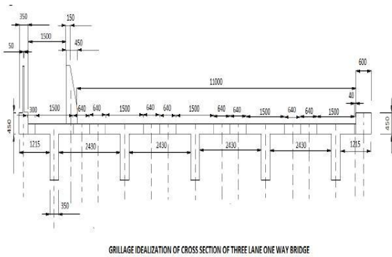
GRILLAGE IDEALIZATION OF CROSS SECTION OF THREE LANE ONE WAY BRIDGE
