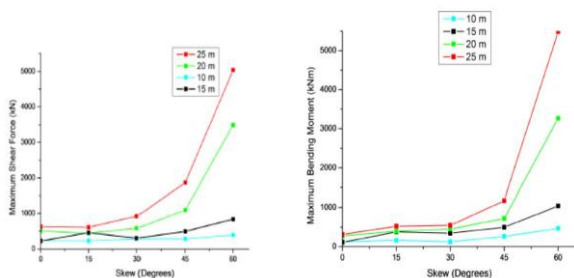
Fig 6: Maximum Shear Force Class70RW+A and Maximum BM Class70RW+A
