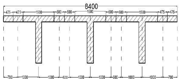
Fig 1: Division of Bridge Cross-Section Into Equivalent Grillage
