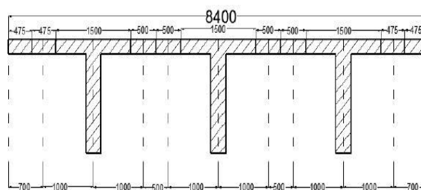
Fig 1: Division of Bridge Cross-Section Into Equivalent Grillage
