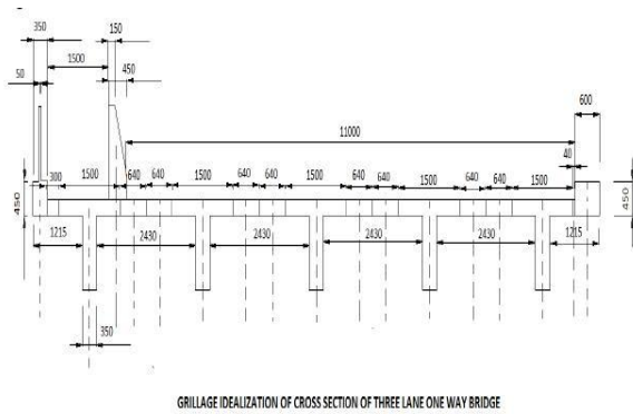
Fig 2: Grillage Idealization of the cross section of bridge. All dim in mm
