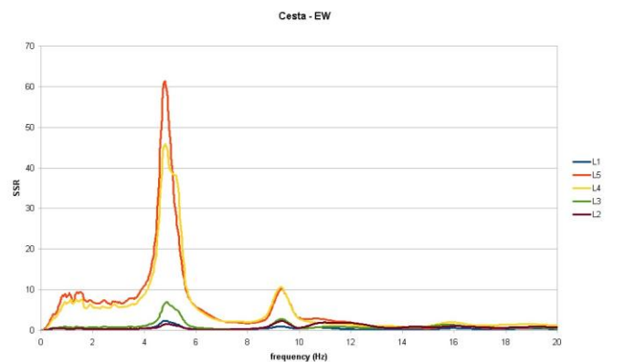
Fig. 13. SSR curves (R9 as reference measurements), Cesta tower, E-W direction
