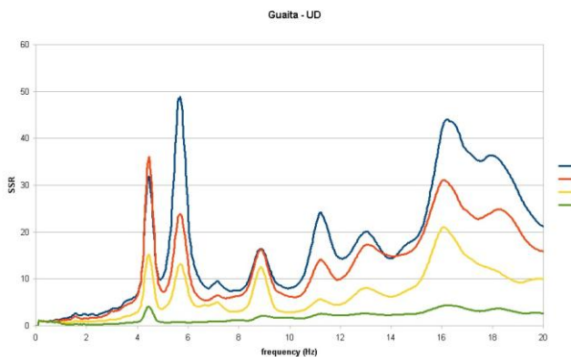
Fig. 11. SSR curves (R15 as reference measurements), Guaita tower, U-D direction
