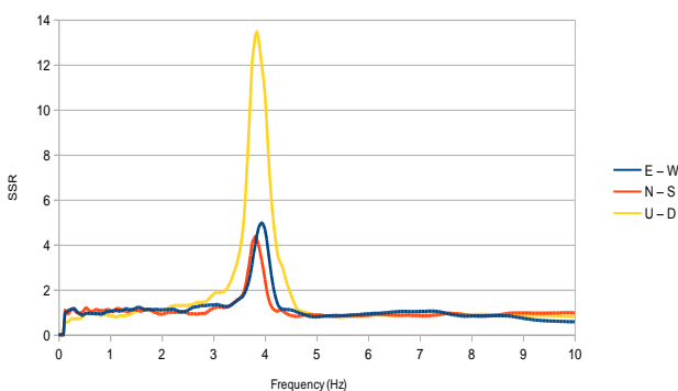
Fig. 15. SSR curves (R7 as reference measurements), Montale tower, N-S direction
