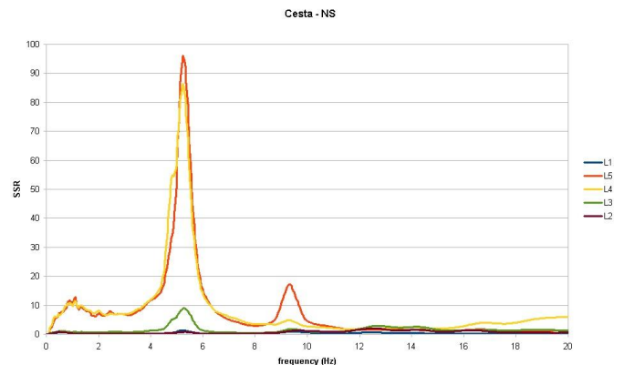
Fig. 12. SSR curves (R9 as reference measurements), Cesta tower, N-S direction
