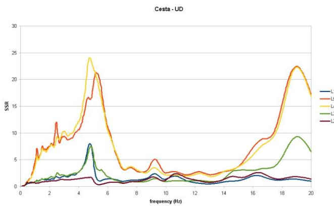
Fig. 14. SSR curves (R9 as reference measurements), Cesta tower, U-D direction
