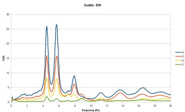
Fig. 10. SSR curves (R15 as reference measurements), Guaita tower, E-W direction
