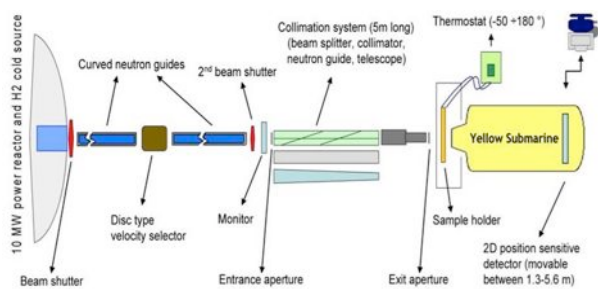
Fig. 2. SANS facility of the BNC
