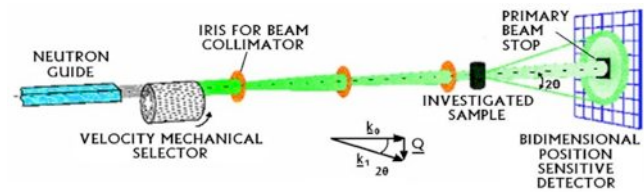
Fig. 1. Scheme of the SANS technique
