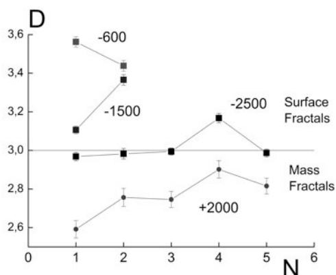
Fig. 10. The magnitudes of the exponents D(N) vs. the numbers of the samples of materials. Evolution of structural properties of linen materials vs. their age.
