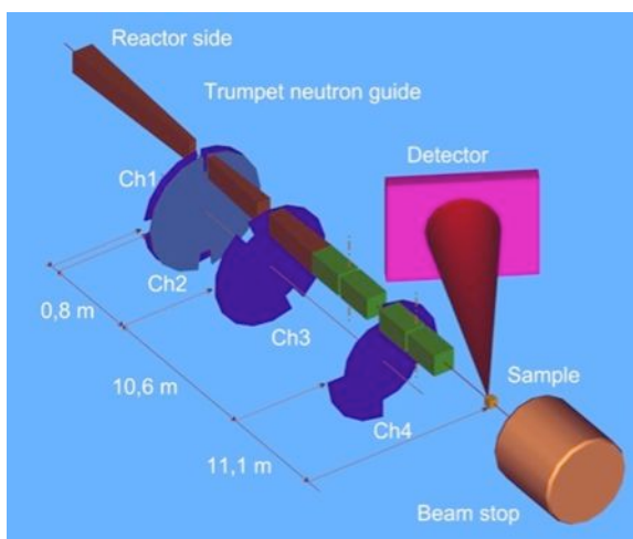
Fig. 3. Scheme of the TOF instrument at the BNC
