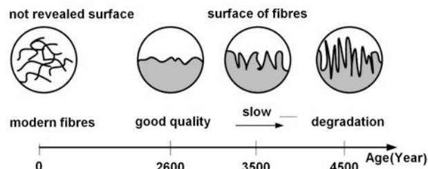
Fig. 11. Evolution of structural properties of linen materials vs. their age.
