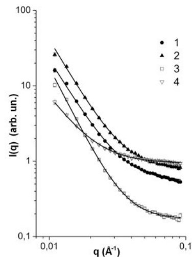
Fig. 9. Scattering intensities for ancient samples dating in the period 2590-2180 B.C. Lines are fitting functions (1)
