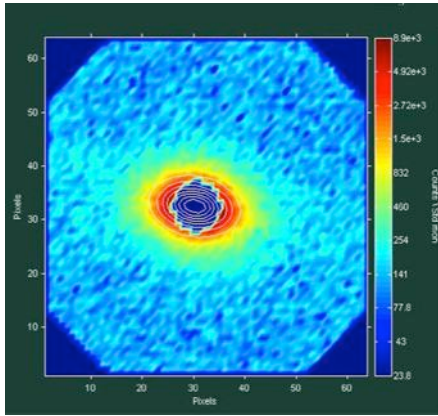
Fig. 6. SANS spectrum from dull wool
