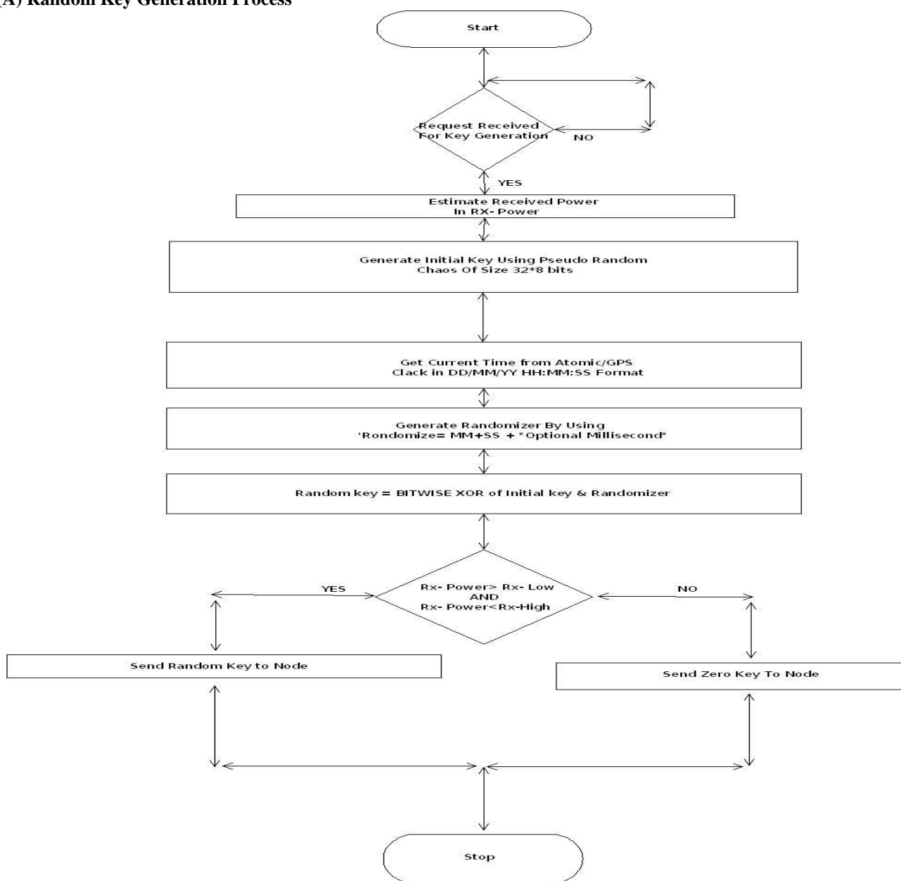
Fig 1 Random Key Generation Process
